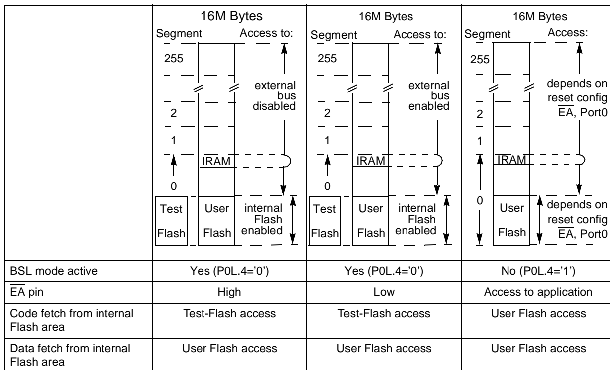
Figure 7 : Memory Configuration after Reset
