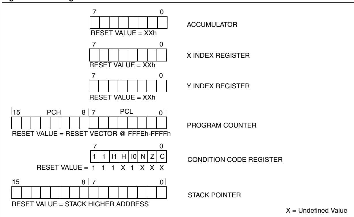
Figure 13. CPU Registers
