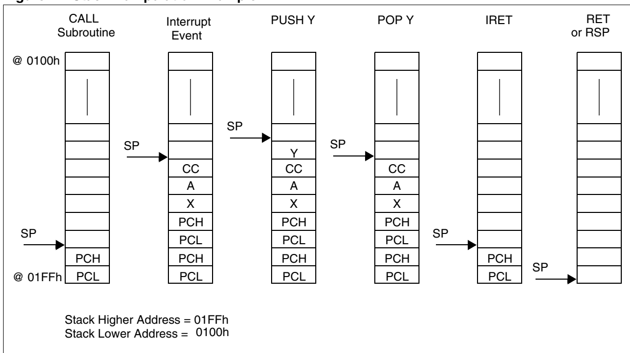
Figure 14. Stack Manipulation Example
