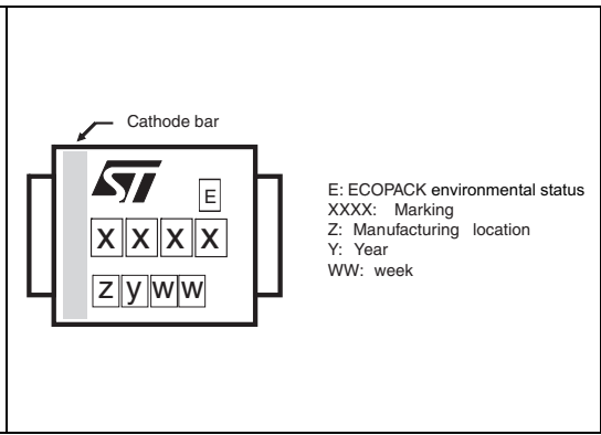
Figure 12. Marking layout
