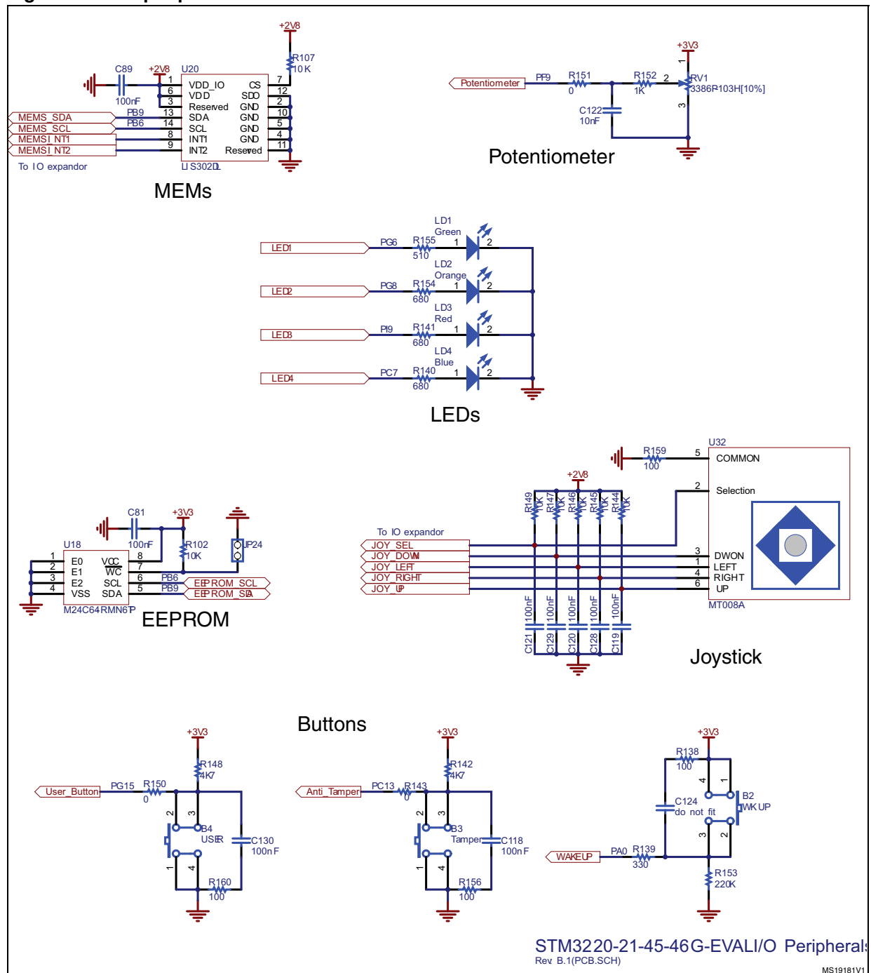
Figure 29. I/O peripherals
