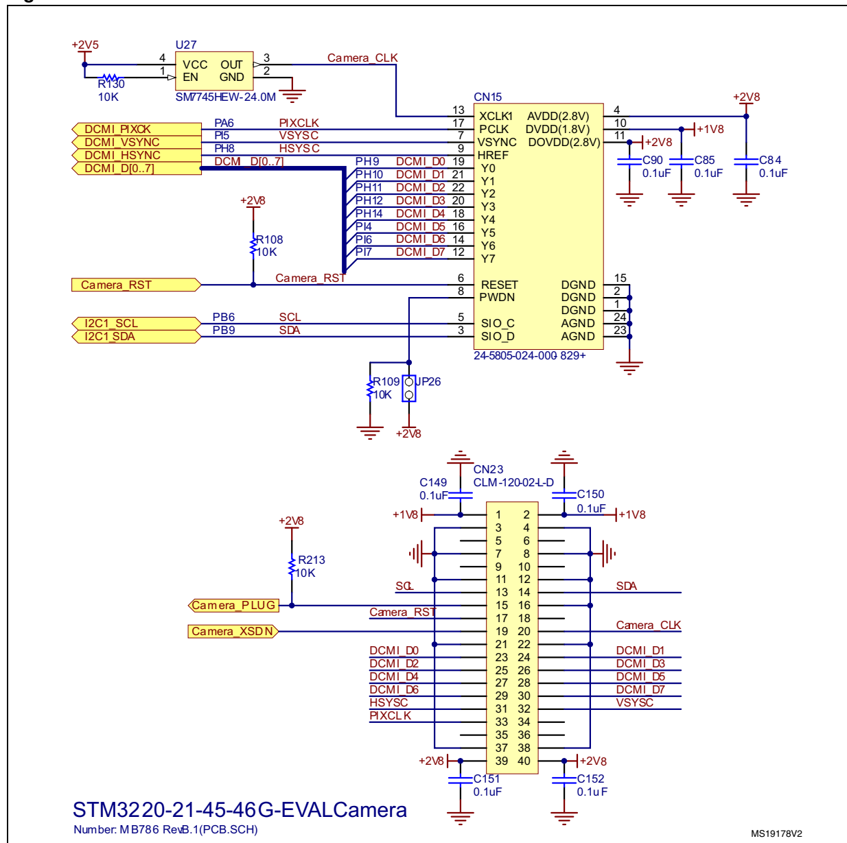
Figure 19. Camera
