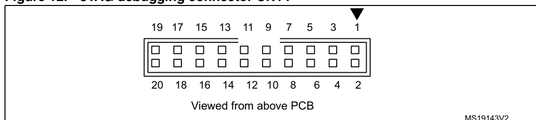
Figure 12. JTAG debugging connector CN14
