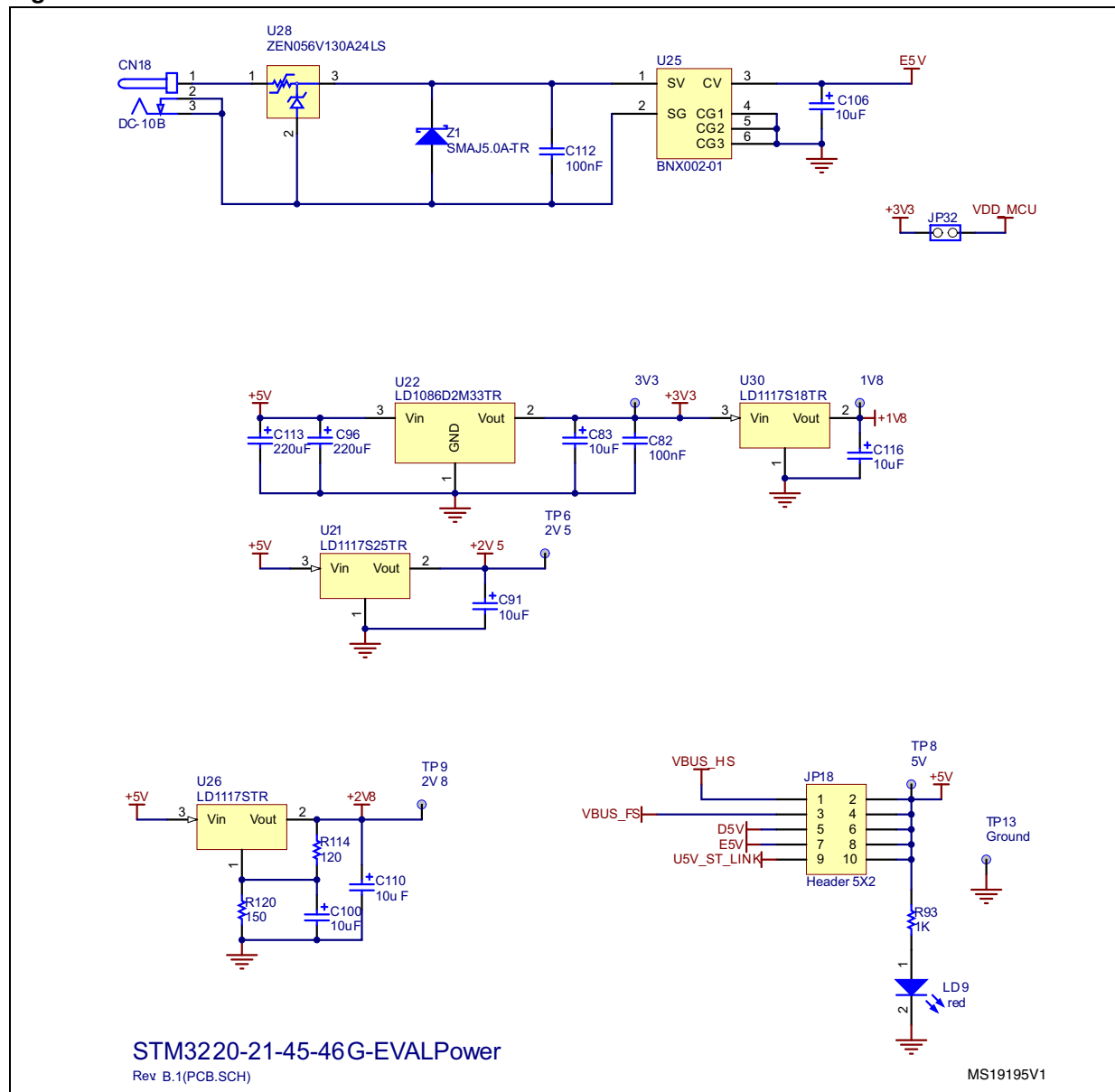
Figure 35. Power
