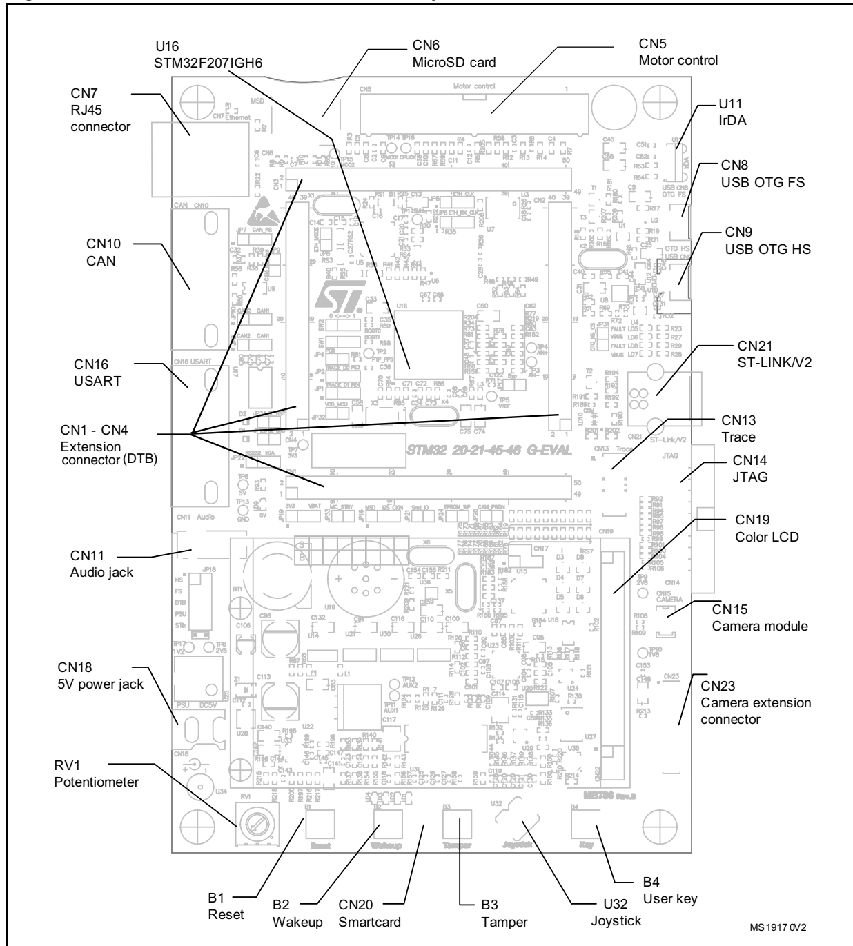
Figure 3. STM3220G-EVAL evaluation board layout
