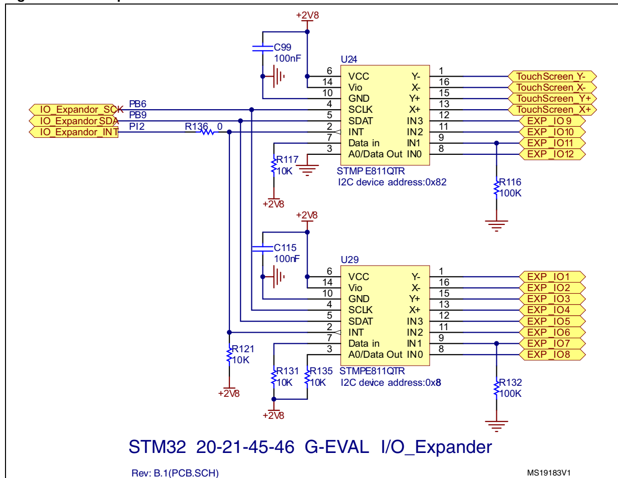
Figure 30. I/O expander
