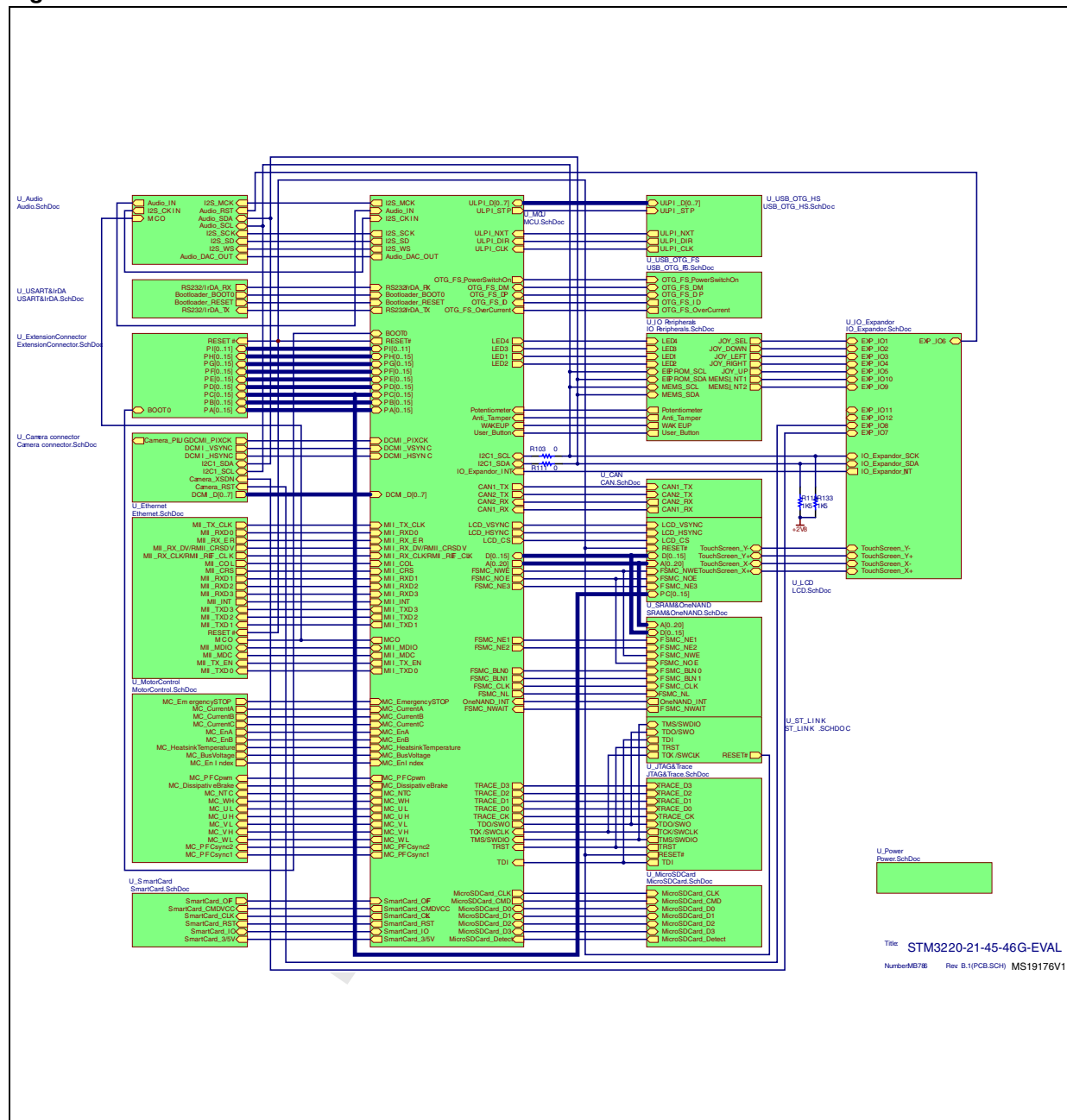
Figure 17. STM3220G-EVAL
