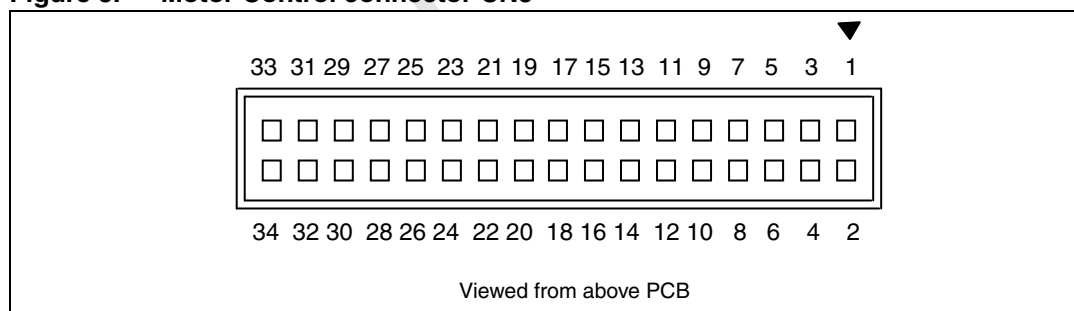
Figure 5. Motor Control connector CN5
