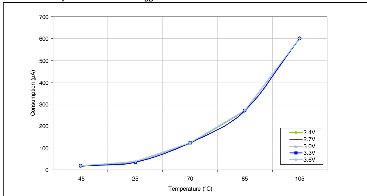
Figure 15. Current consumption in Stop mode with regulator in run mode versus temperature at different V_{DD} values
