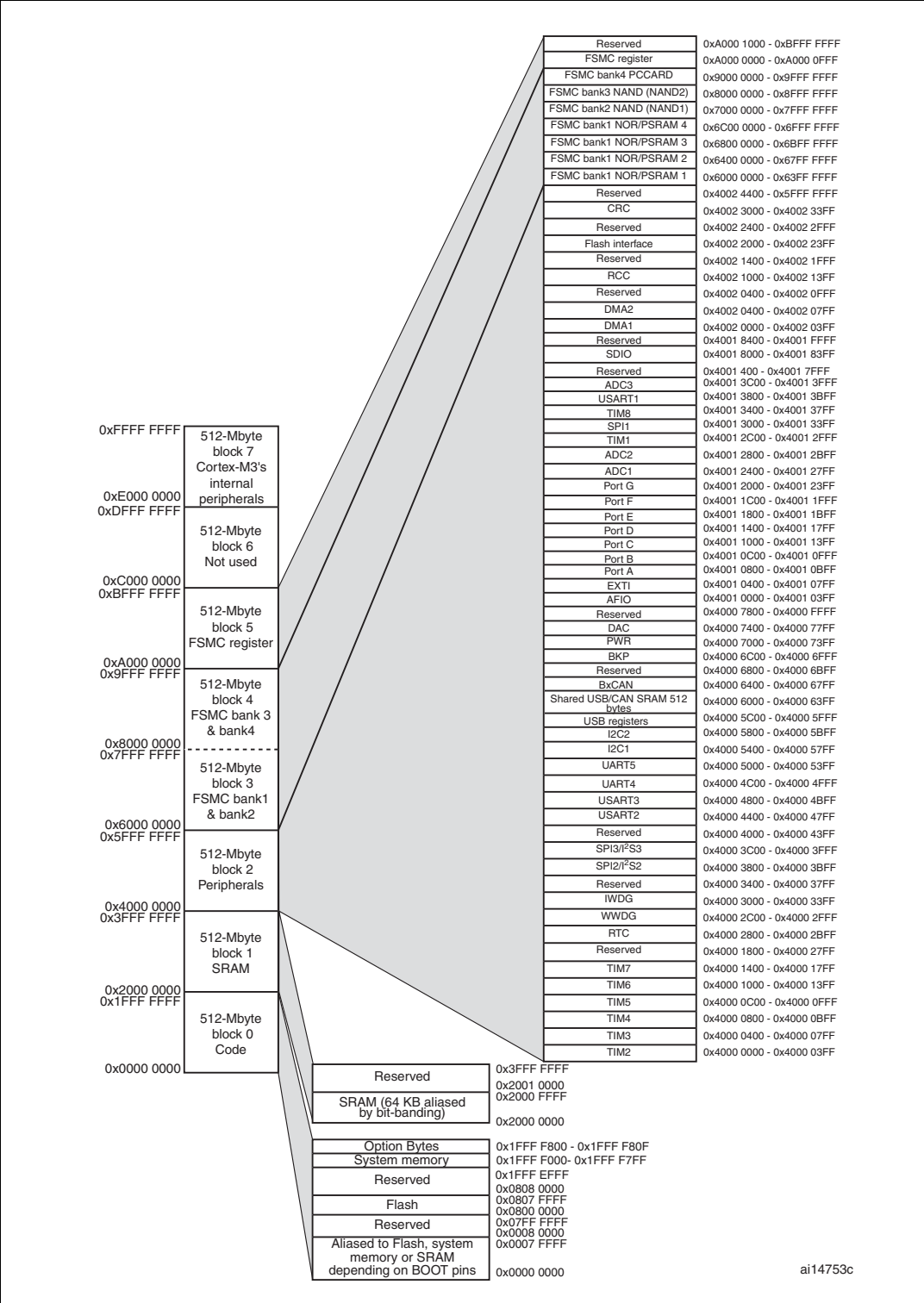
Figure 8. Memory map
