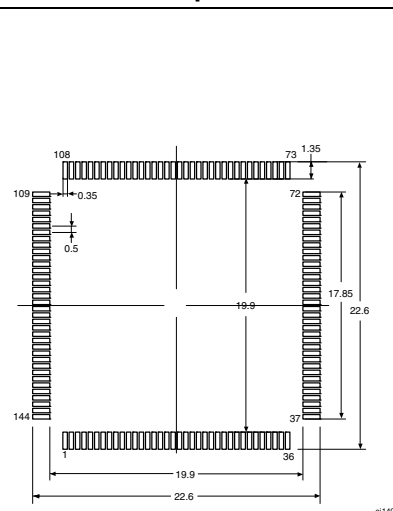
Figure 56. Recommended footprint (1)(2)
