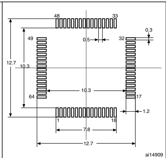
Figure 62. Recommended footprint (1)(2)
