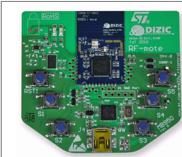
Figure 1. MB950 RF-mote board
