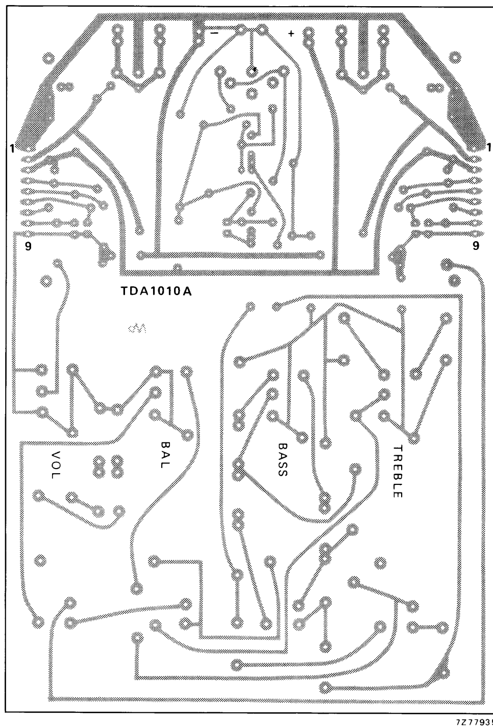
Fig.18 Track side of printed-circuit board used for the circuit of Fig.17 (Fig.16 partly); p.c. board dimensions 169 mm x 118 mm.
