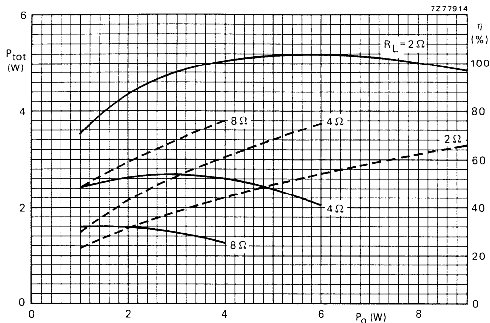
Fig.7 Total power dissipation (solid lines) and the efficiency (dashed lines) of the circuit of Fig.3 as a function of the output power with the load impedance as a parameter (for R_L = 2 \Omega an external bootstrap resistor of 220 \Omega has been used); typical values. V_P = 14,4 \text{ V} ; f = 1 \text{ kHz} .
