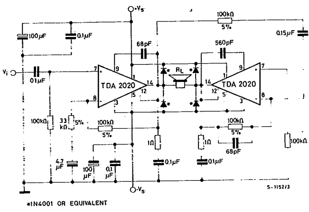
Fig. 18 - 30W bridge amplifier configuration with split power supply ( R_L = 8 \Omega d \leq 1\% ; V_s = \pm 17V )
