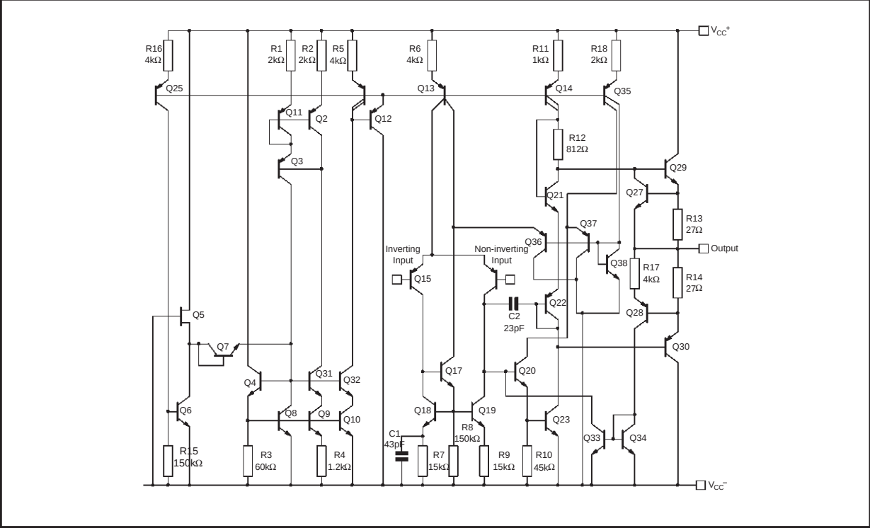
SCHEMATIC DIAGRAM (1/2 TDA2320A)
