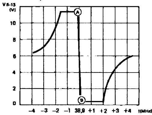
Fig. 4 — AFC VOLTAGE VERSUS FREQUENCY V 5-13
