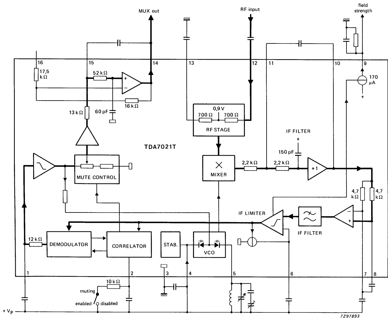
Fig.1 Block diagram.
