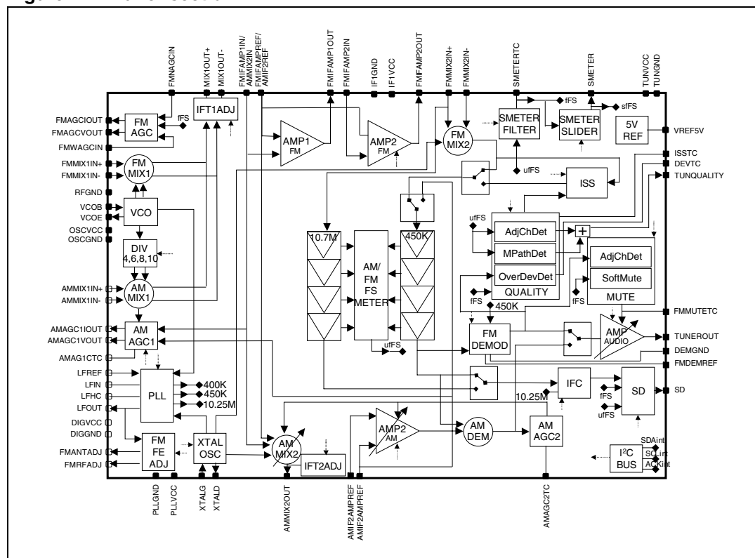
Figure 1. Tuner section
