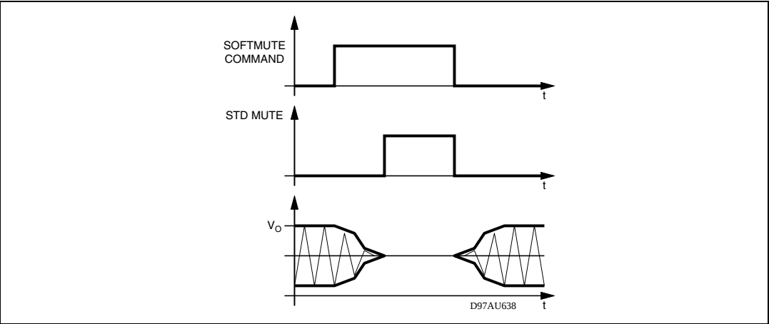
Figure 15. Signal during stereo decoder's softmute
