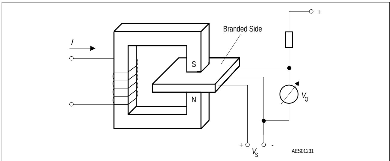
Figure 3 Sensor/Magnetic-Field Configuration
