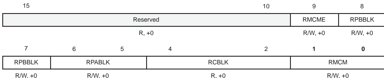
Figure 3–12. Multichannel Control Register 1x (MCR1x)
