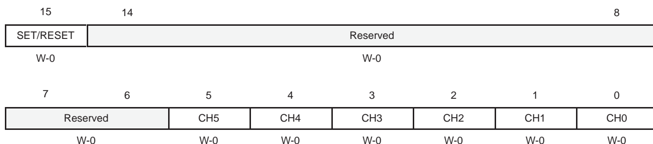
Figure 3–19. DMA Channel Enable Control Register (DMCECTL)
