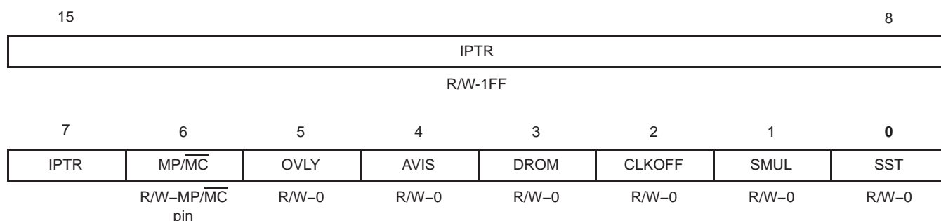
Figure 3–4. Processor Mode Status Register (PMST)
