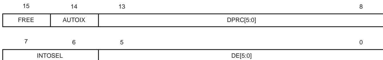
Figure 3–22. DMPREC Register
