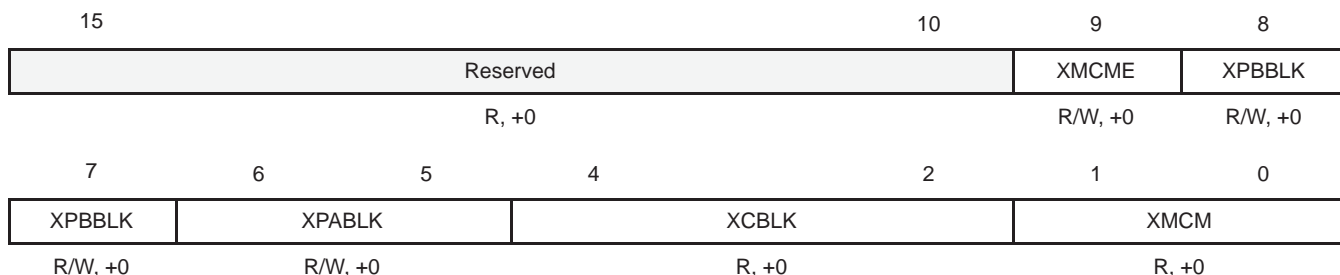
Figure 3–11. Multichannel Control Register 2x (MCR2x)
