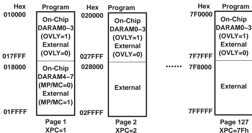
Figure 3–3. Extended Program Memory Map
