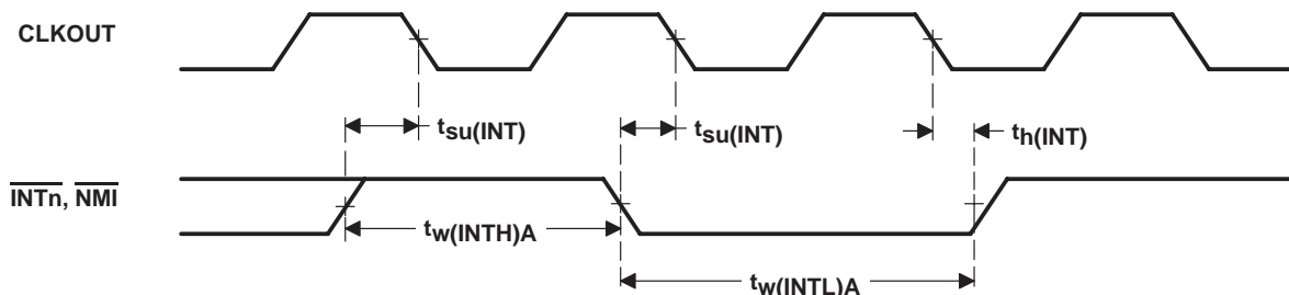
Figure 28. Interrupt Timing
