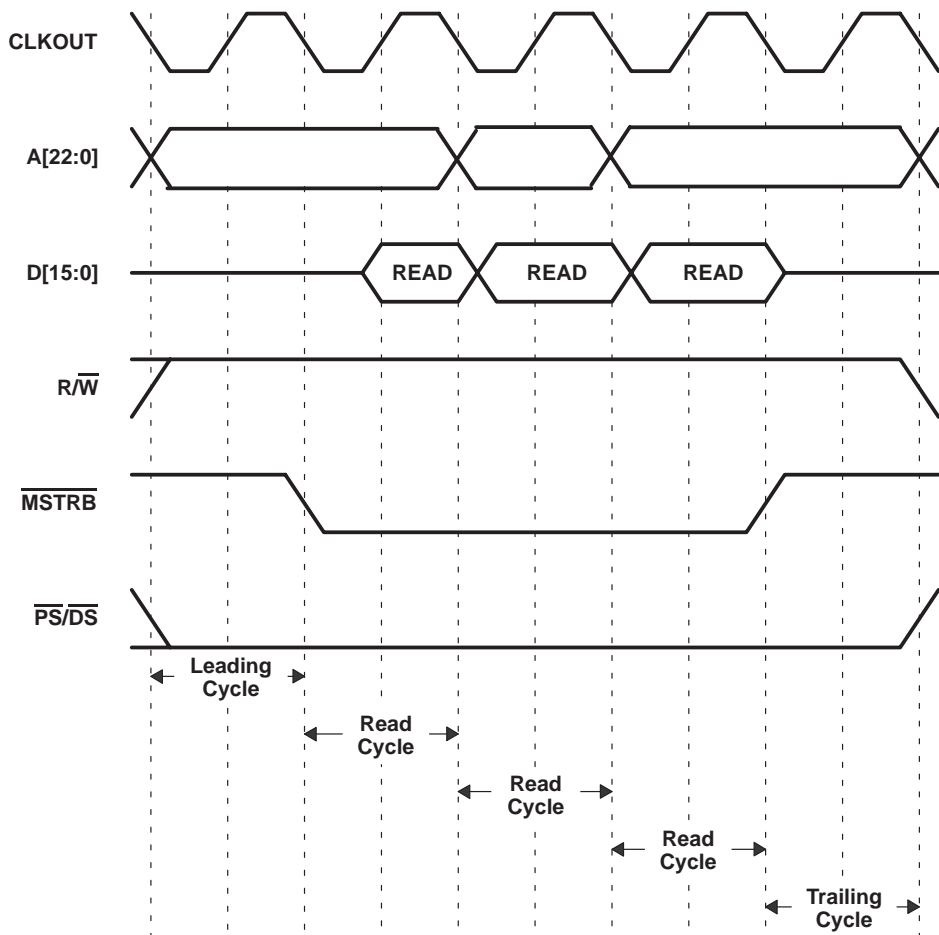
Figure 9. Consecutive Memory Read Bus Sequence (n = 3 reads)
