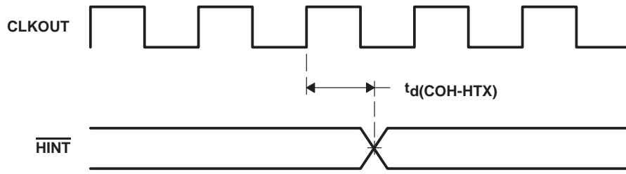
Figure 42. \overline{\text{HINT}} Timing
