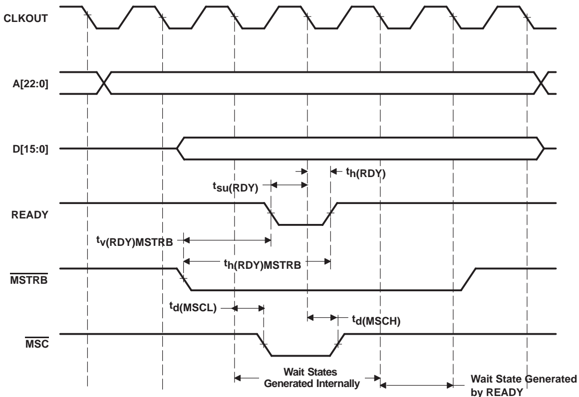
Figure 23. Memory Write With Externally Generated Wait States
