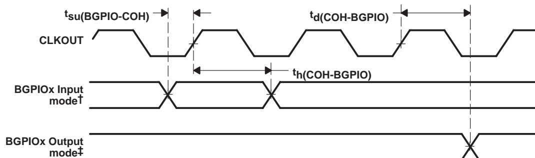
Figure 35. McBSP General-Purpose I/O Timings
