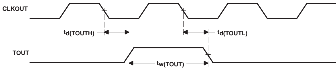
Figure 32. TOUT Timing
