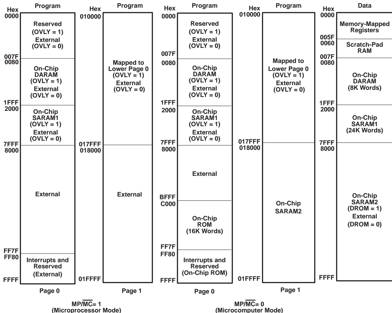
Figure 1. Memory Map
