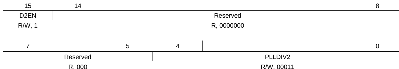
Figure 3-19. PLL Divider 2 Register Layout (0x1C8E)
