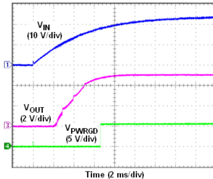
Figure 32. Start-Up Sequence
