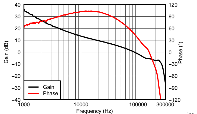
Figure 7. V_{OUT} = 3.3\text{ V} , I_{OUT} = 2\text{ A} , C_{OUT1} = 44\text{ }\mu\text{F} ceramic, C_{OUT2} = 56\text{ }\mu\text{F} electrolytic, f_{SW} = 400\text{ kHz}
