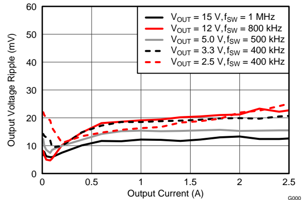
Figure 9. Voltage Ripple vs. Output Current
