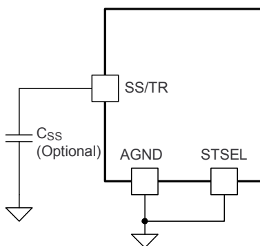
Figure 36. Slow Start Capacitor ( C_{SS} ) and STSEL Connection
