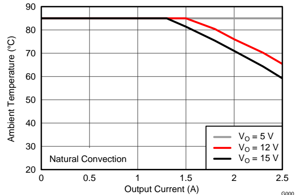
Figure 23. Safe Operating Area
