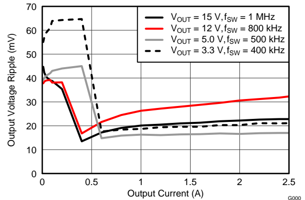
Figure 21. Voltage Ripple vs. Output Current
