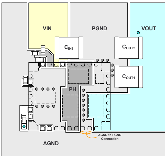
Figure 41. Typical Top-Layer Recommended Layout
