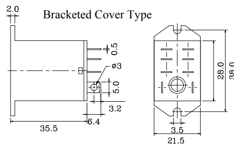
DPDT (2C)
