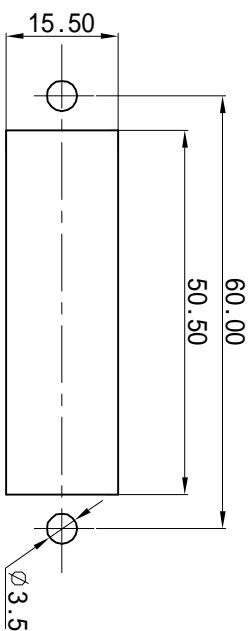
PANEL CUT OUT
